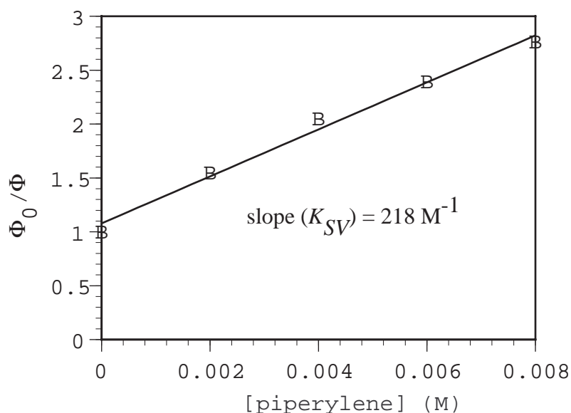
Fig. Stern-Volmer plot for photolysis of 1 in 50% THF-H 2 O at 350 nm.
